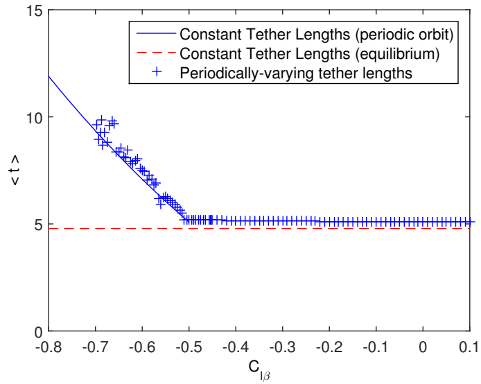
Figure 9: Normalized average tension versus C_{l\beta} for wind velocity equal to 10m/s.
