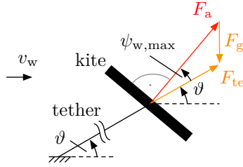
Figure 3: Sketch of a crosswind flying kite with gravity, seen from the side.
